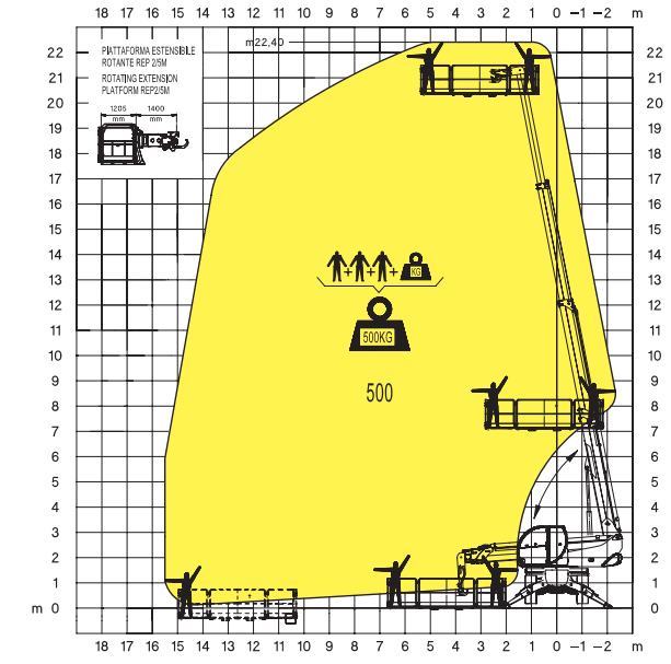
TP 2.10 Telescopisch platform TP 2.10
